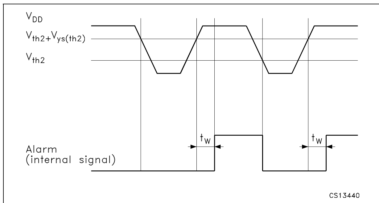
Figure 1 : Alarm as a function of V_{DD} ( t_W = 10\text{ ms} ), V_{THSEL} = V_{DD} or floating
